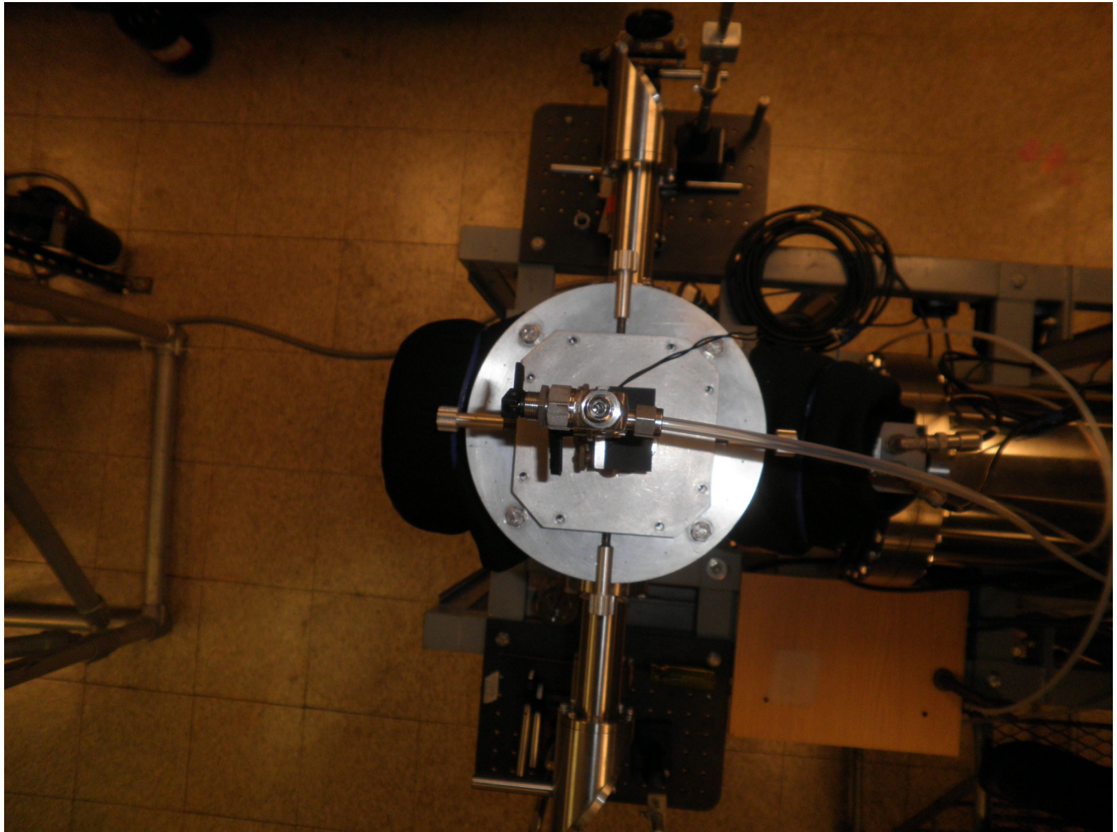
Top view of angular reflectron portion
